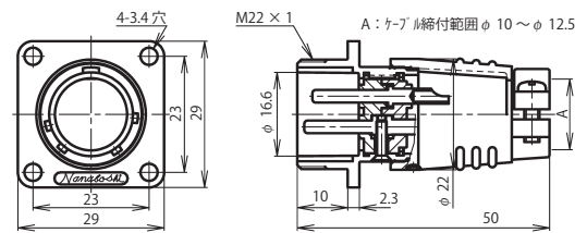
NET-20 ■ -Ad(F)M
